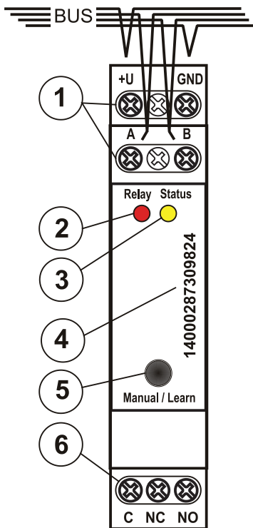
Figure: 1 = bus terminals (CC-01(02) cable): +U red, GND black, A yellow, B green; 2 = red LED – relay triggering; 3 = yellow LED - failure; 4 = production code; 5 = enrollment or manual trigger button; 6 = relay terminal;
